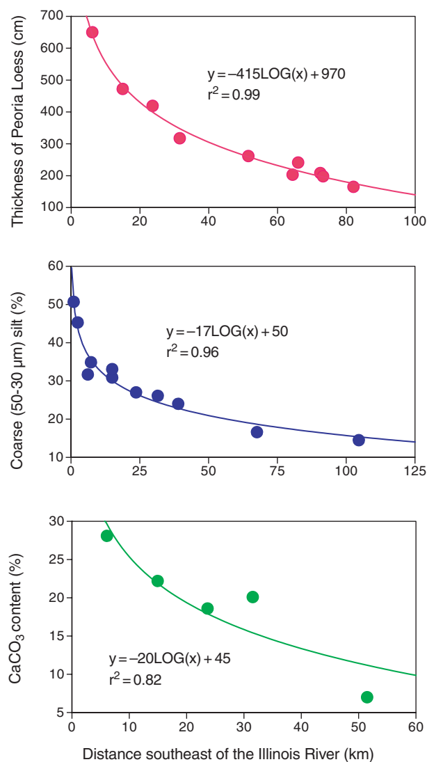
Figure 12 Thickness, coarse silt content, and carbonate content of Peoria (last glacial) Loess as a function of distance southeast of the Illinois River, IL, USA. Data from Smith (1942); regression equations computed by D.R. Muhs.
